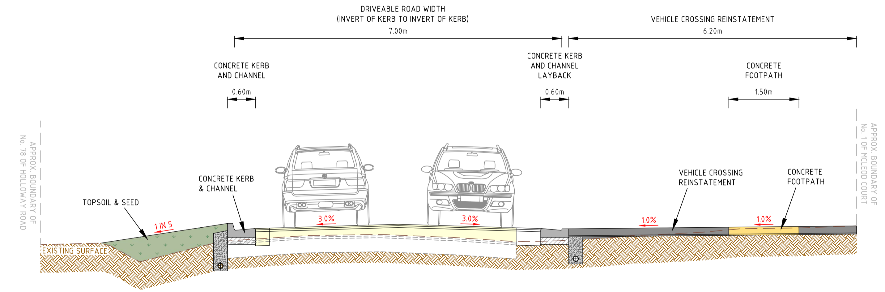
TYPICAL SECTION F-F SCALE 0 0.5 1.0 1.5 2.0 2.5 METRES
