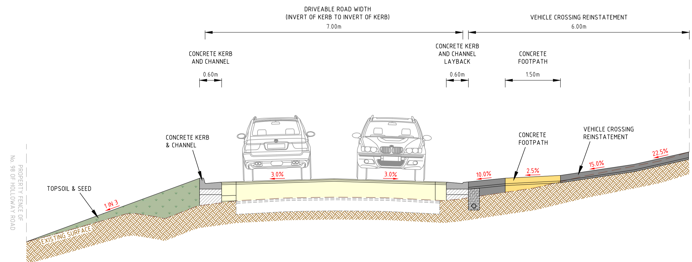
TYPICAL SECTION C-C
