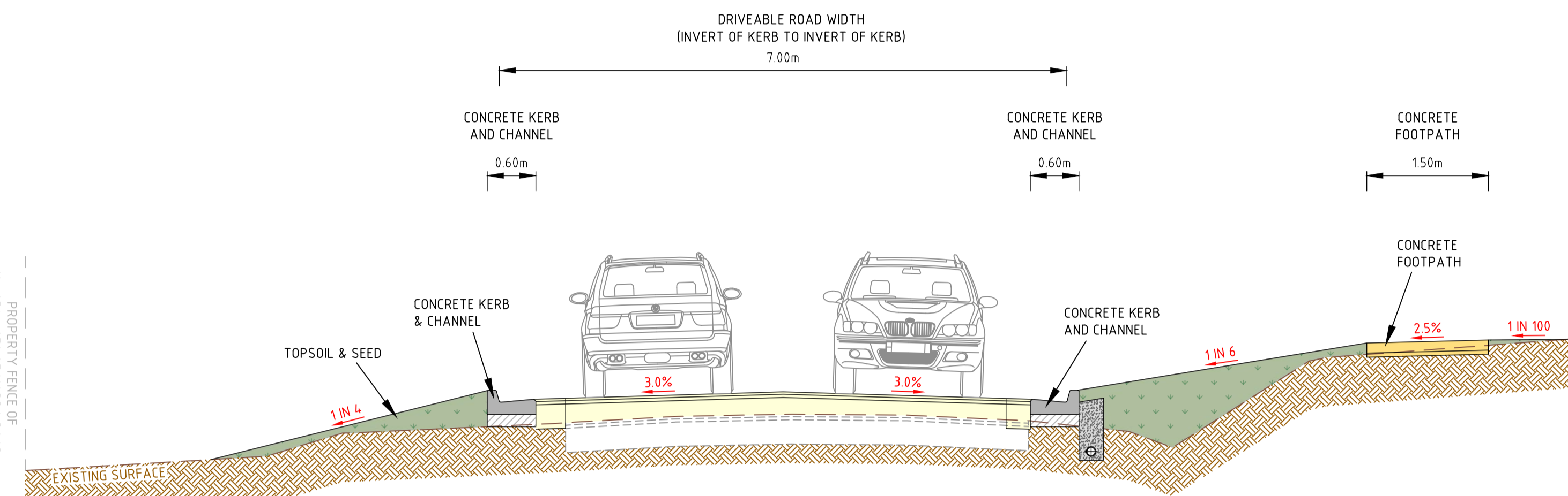
TYPICAL SECTION B-B
