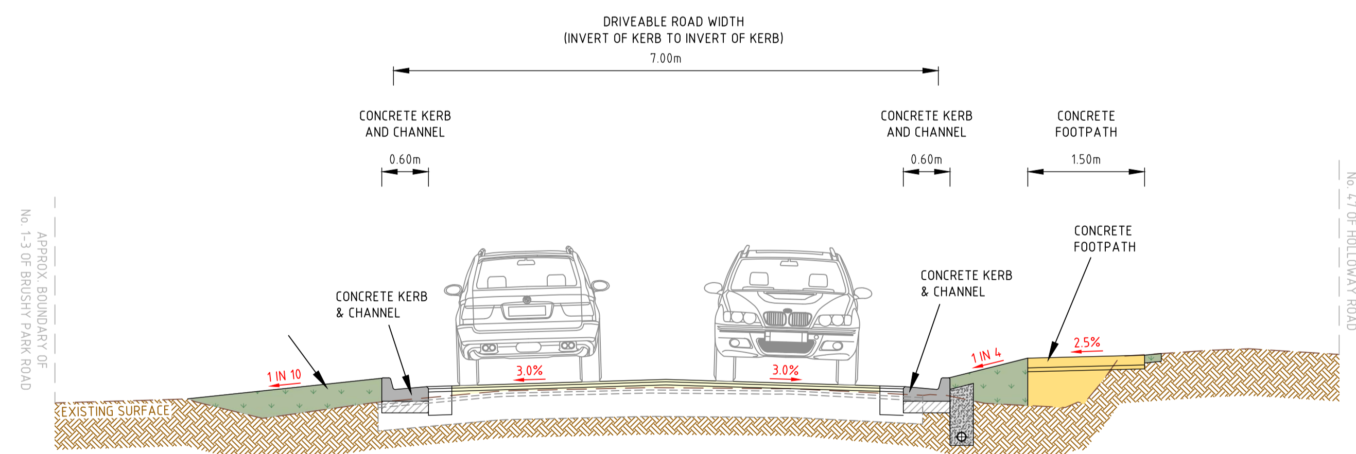
TYPICAL SECTION K-K
