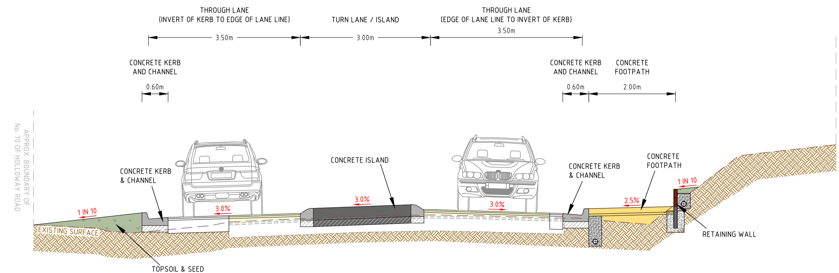
TYPICAL SECTION H-H
