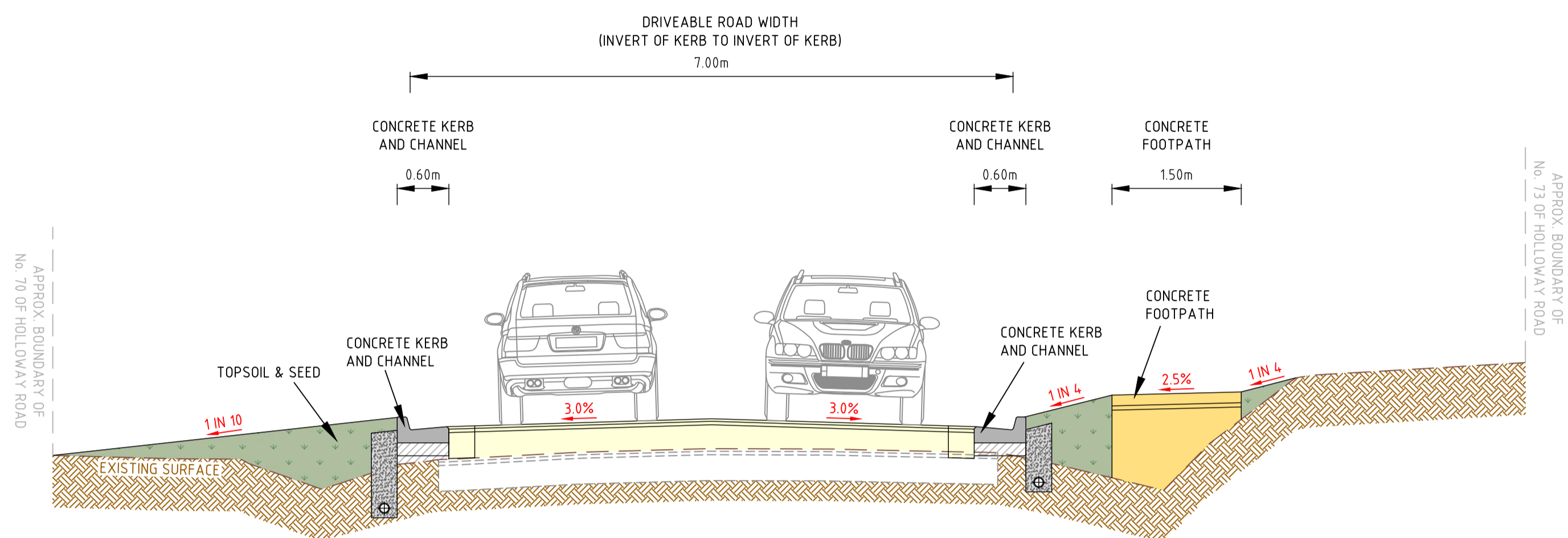
TYPICAL SECTION G-G
