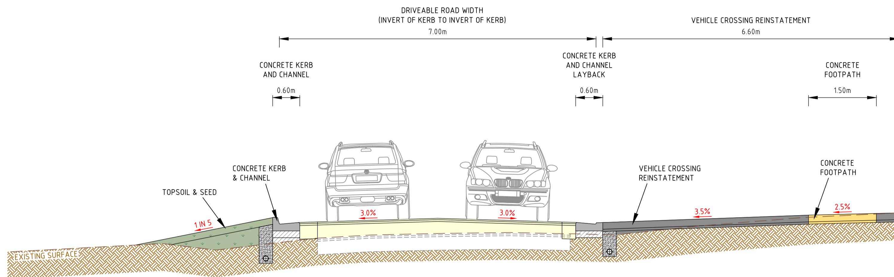
TYPICAL SECTION A-A
