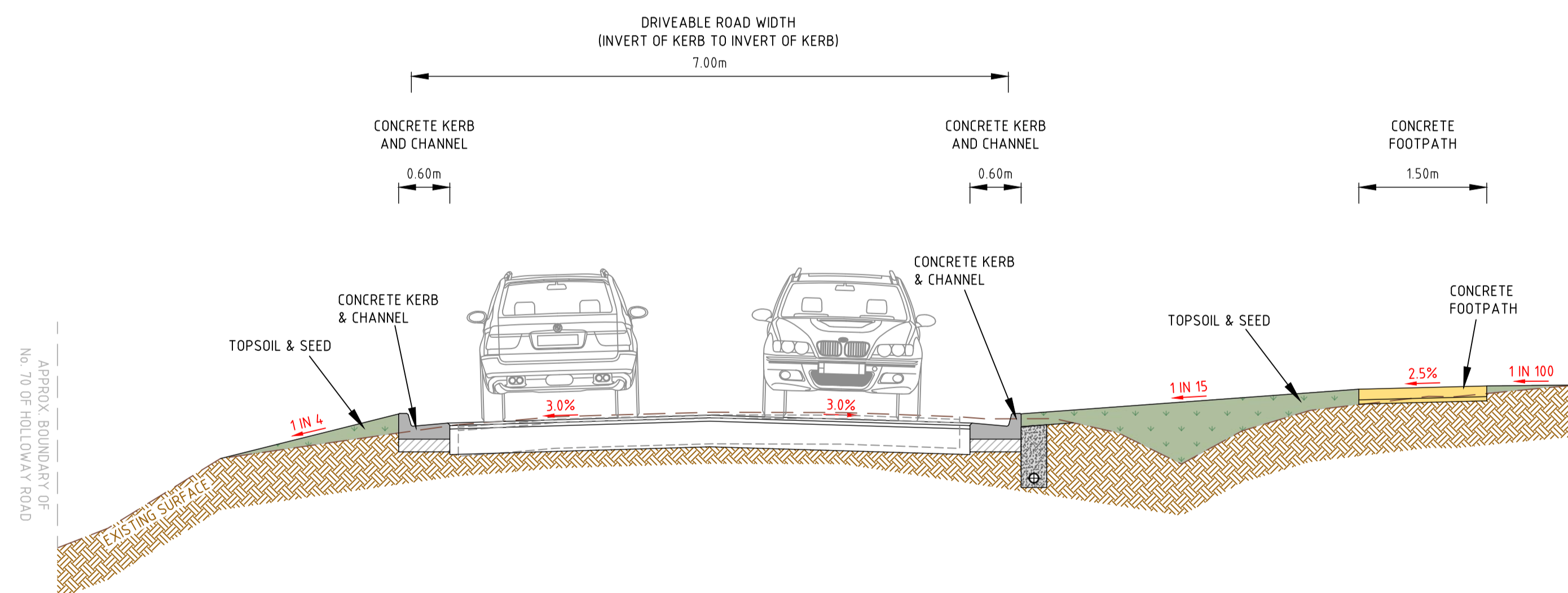
TYPICAL SECTION I-I
